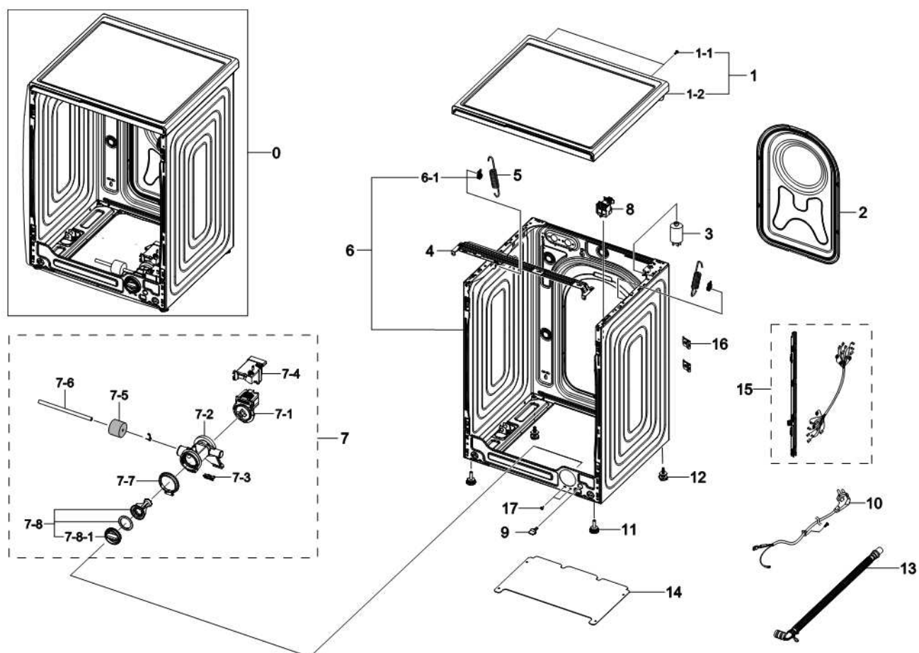
Exploded View
