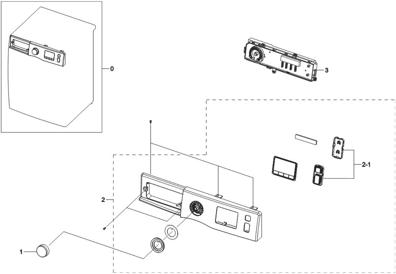
Exploded View
