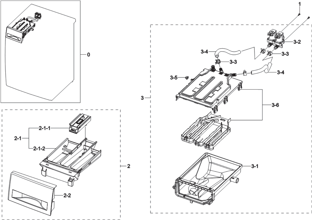
Exploded View
