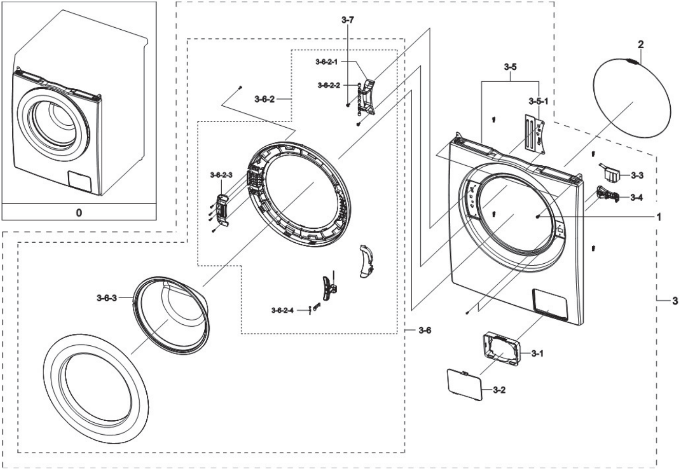
Exploded View
