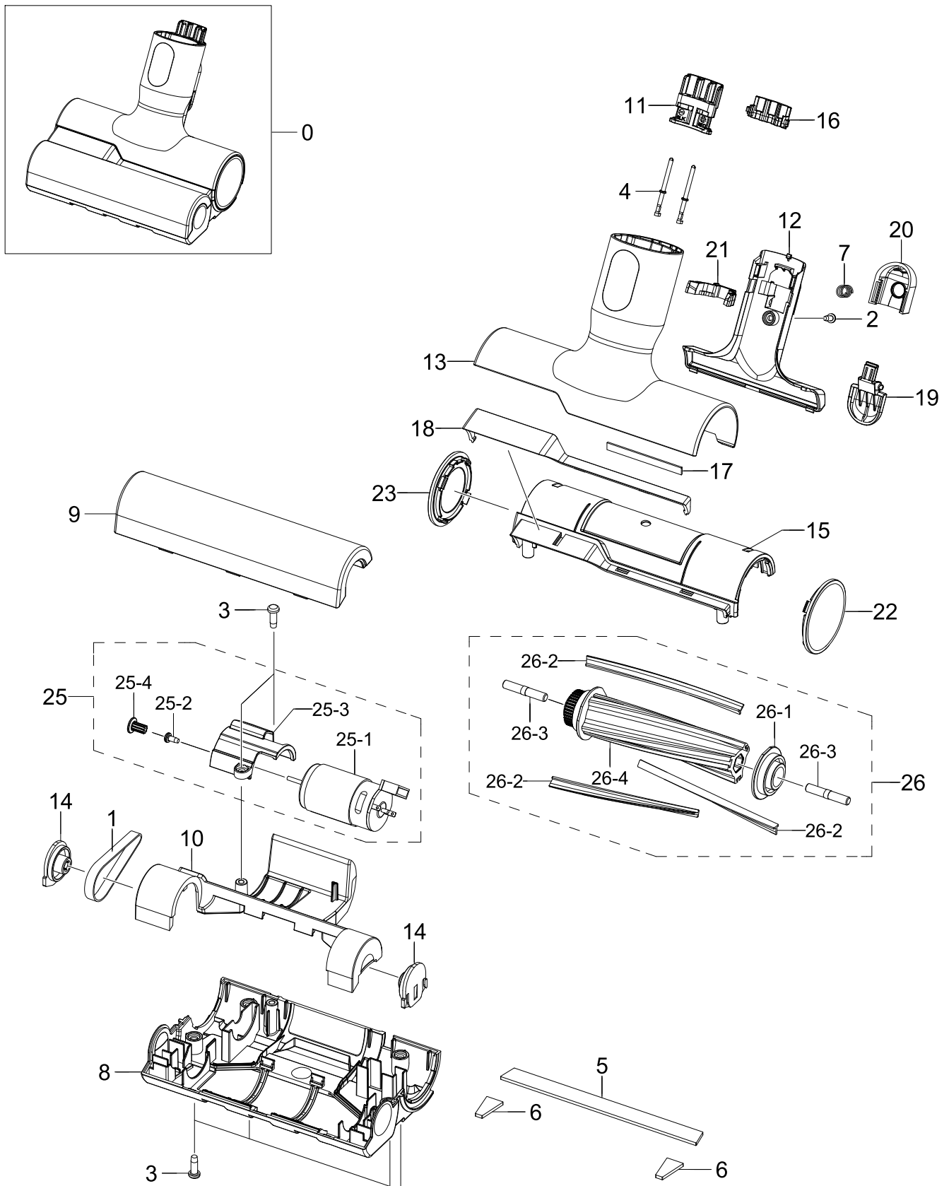
Exploded View
