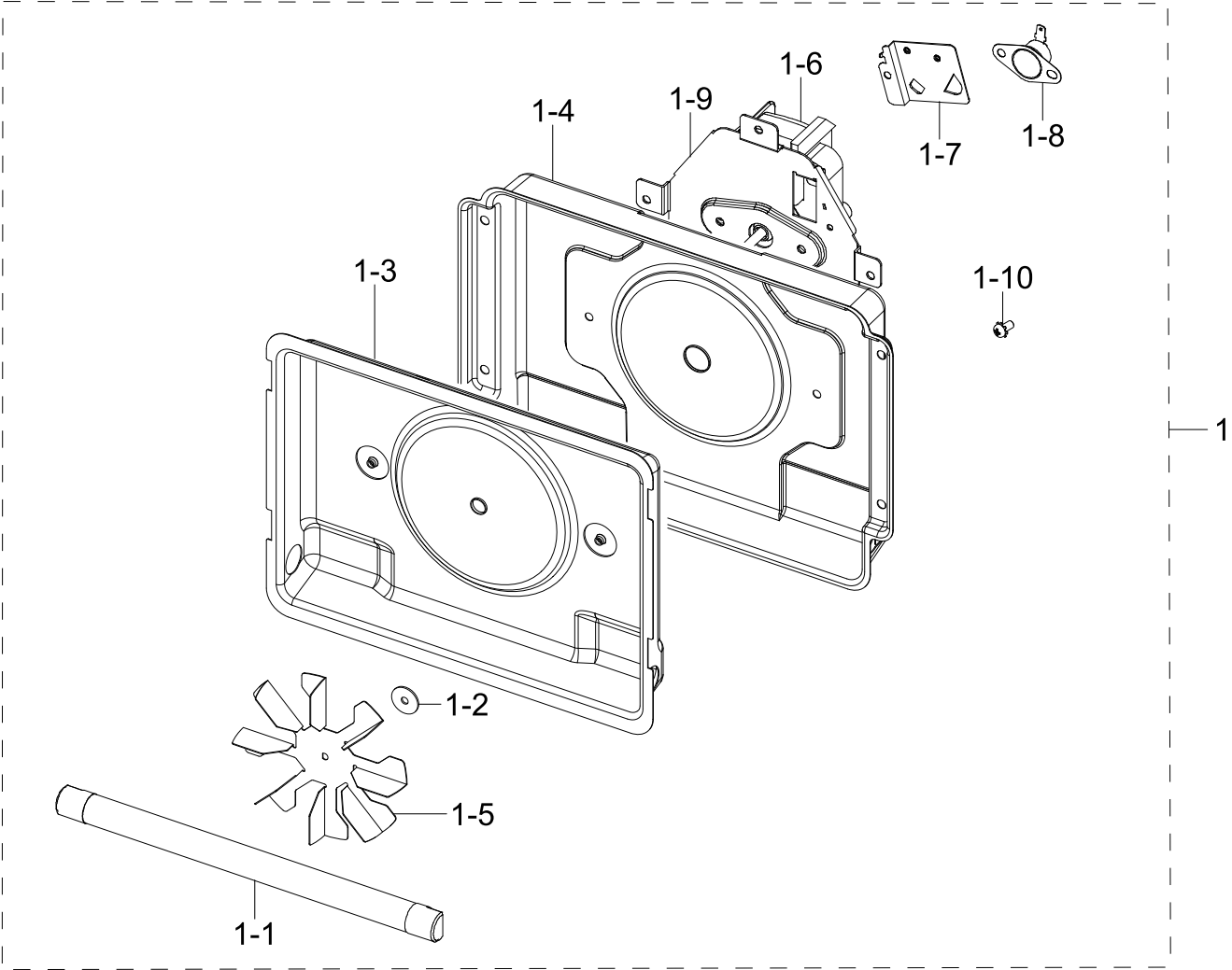
Exploded View
