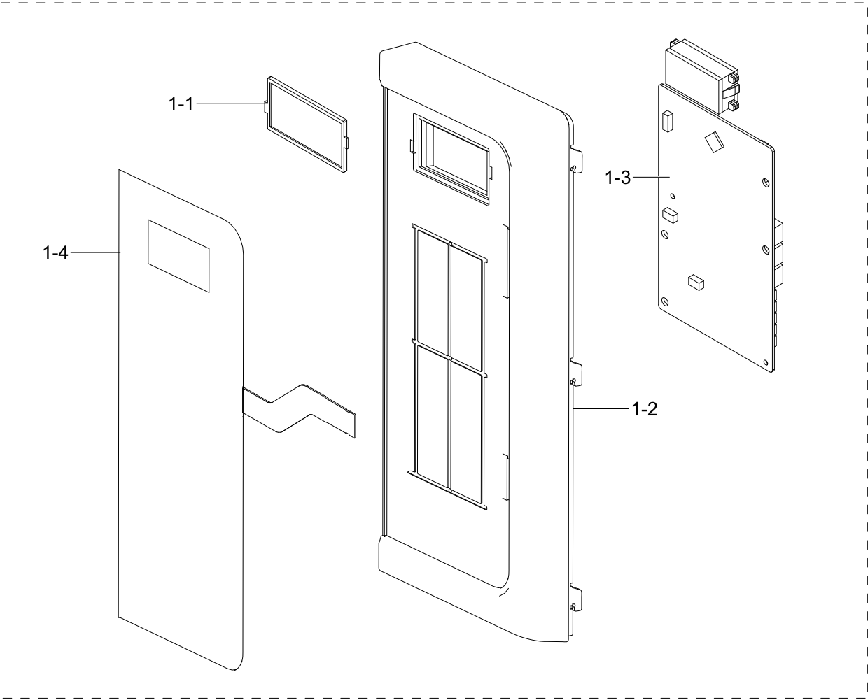
Exploded View
