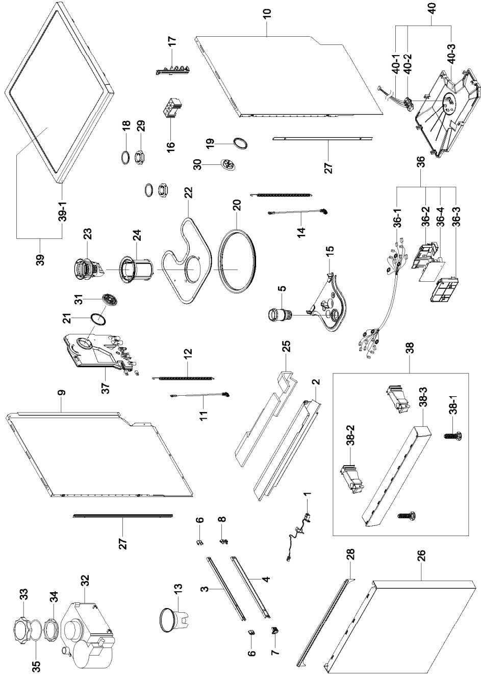
Exploded View
