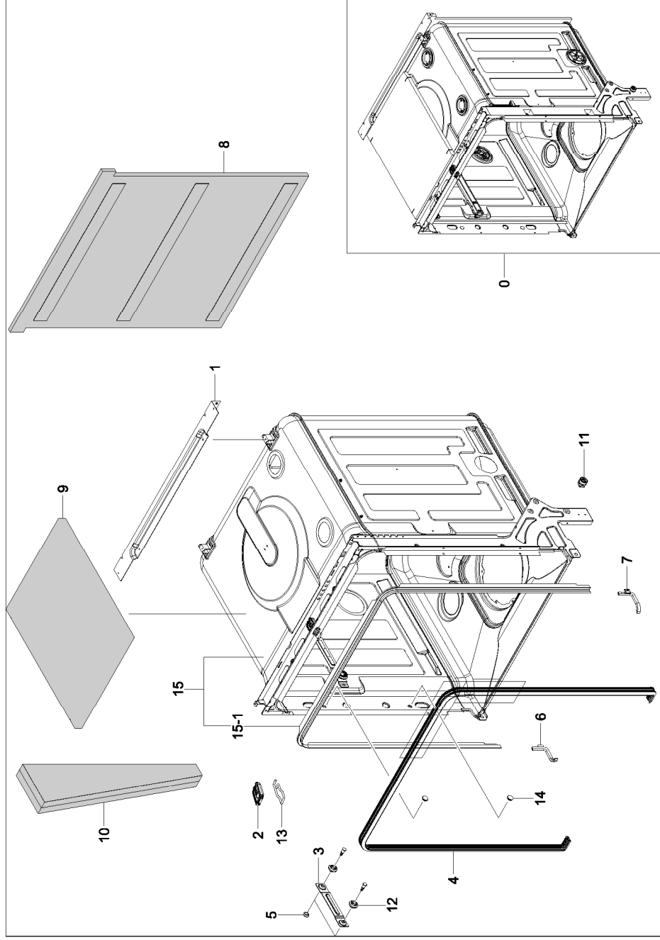
Exploded View
