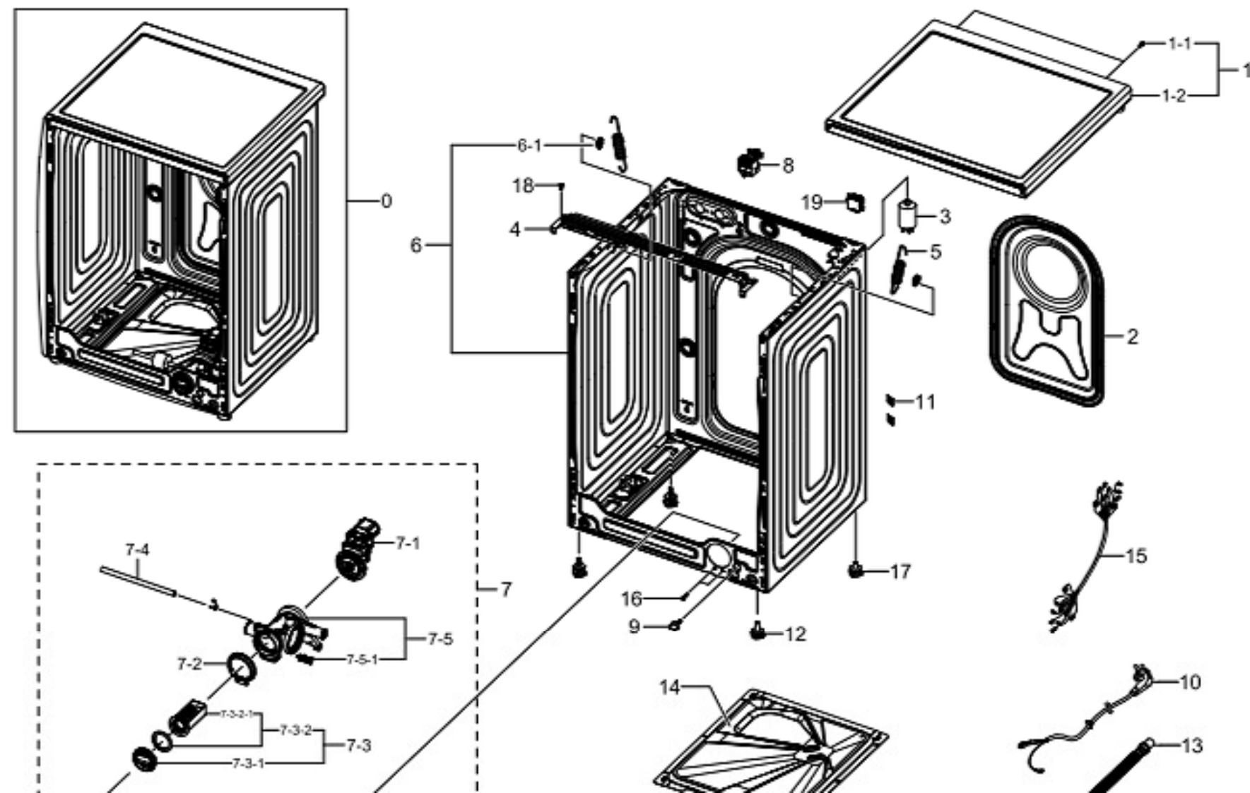
Exploded View
